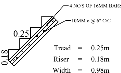
STAIRCASE DETAILS
