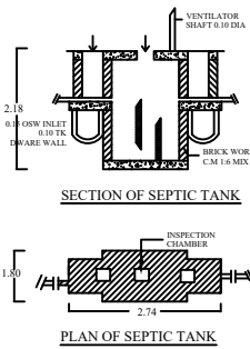
SEPTIC TANK
