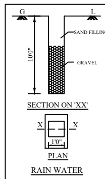
RAINWATER HARVESTING
