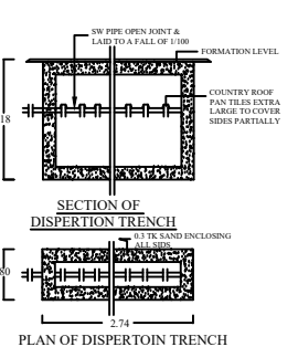
DISPERSION TRENCH
