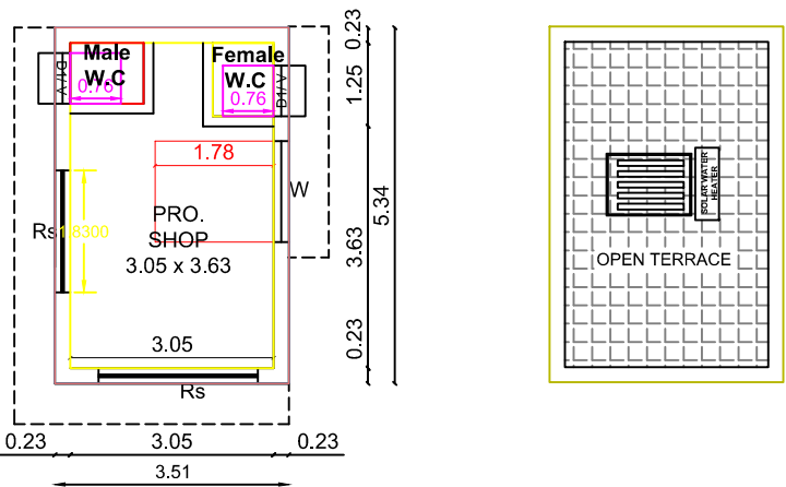
GROUND FLOOR PLAN TERRACE FLOOR PLAN
