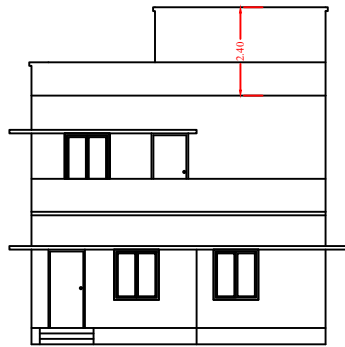
FRONT ELEVATION [FROM NORTH SIDE]
