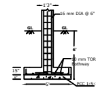
COLUMN FOUNDATION
