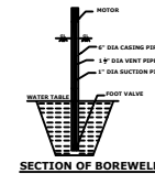
SECTION OF BOREWELL
