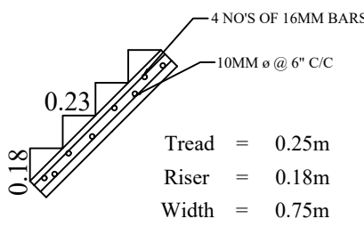
STAIRCASE DETAILS
