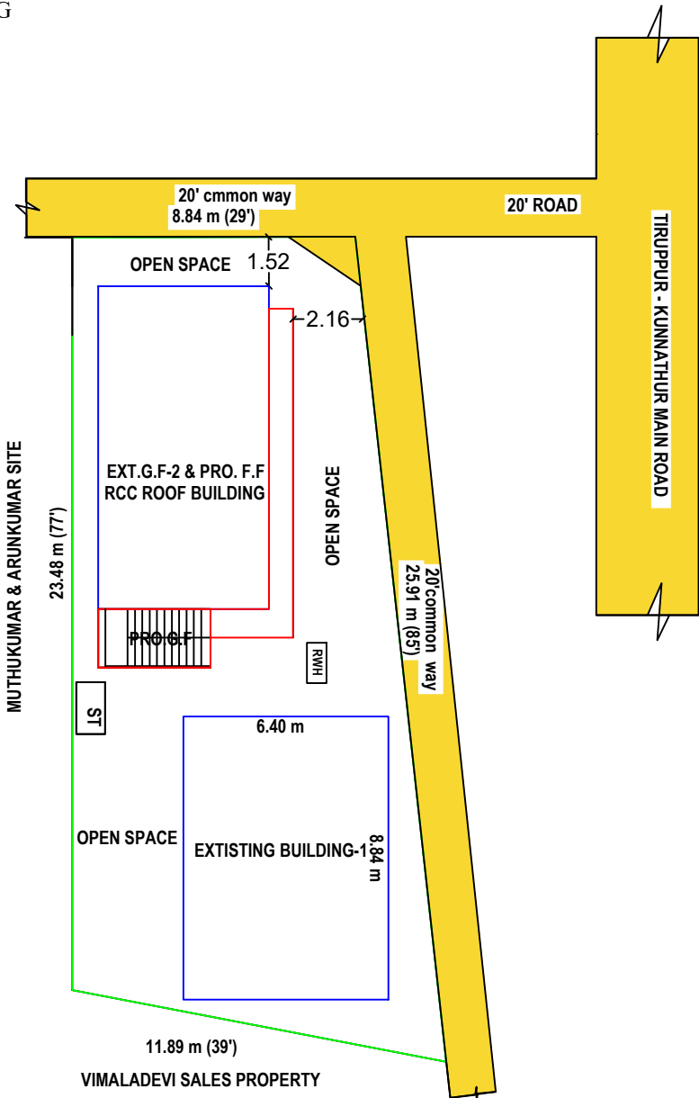
SITE PLAN
