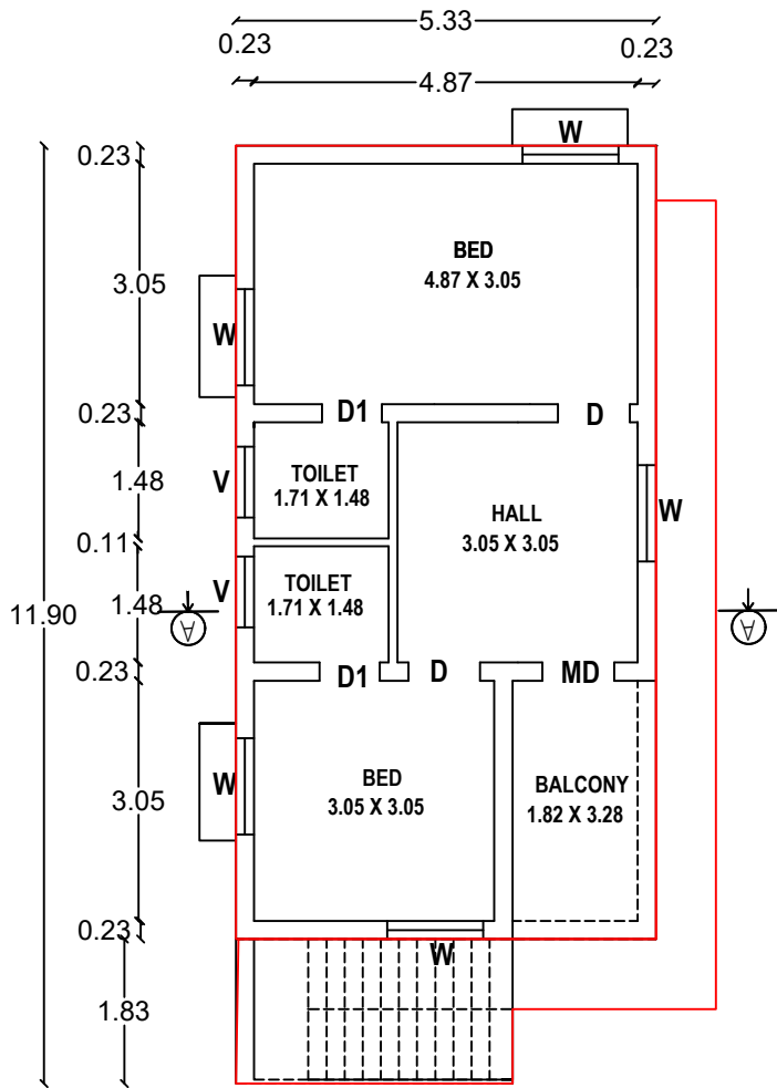
PRO.ADDI.FIRST FLOOR PLAN
