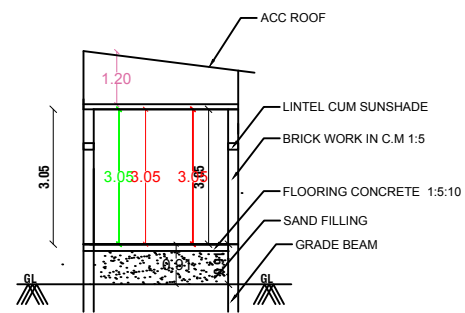
SECTION-AB
