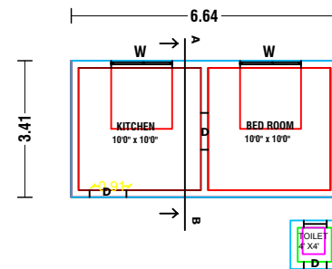
PLAN
