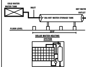
SOLAR HOT WATER SYSTEM DETAILS
