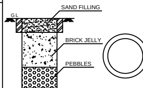
RAIN WATER HARVESTING SYSSTEM
