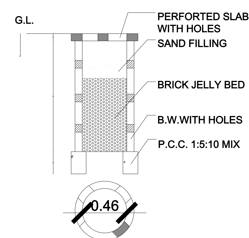
RAIN WATER HARVEST
