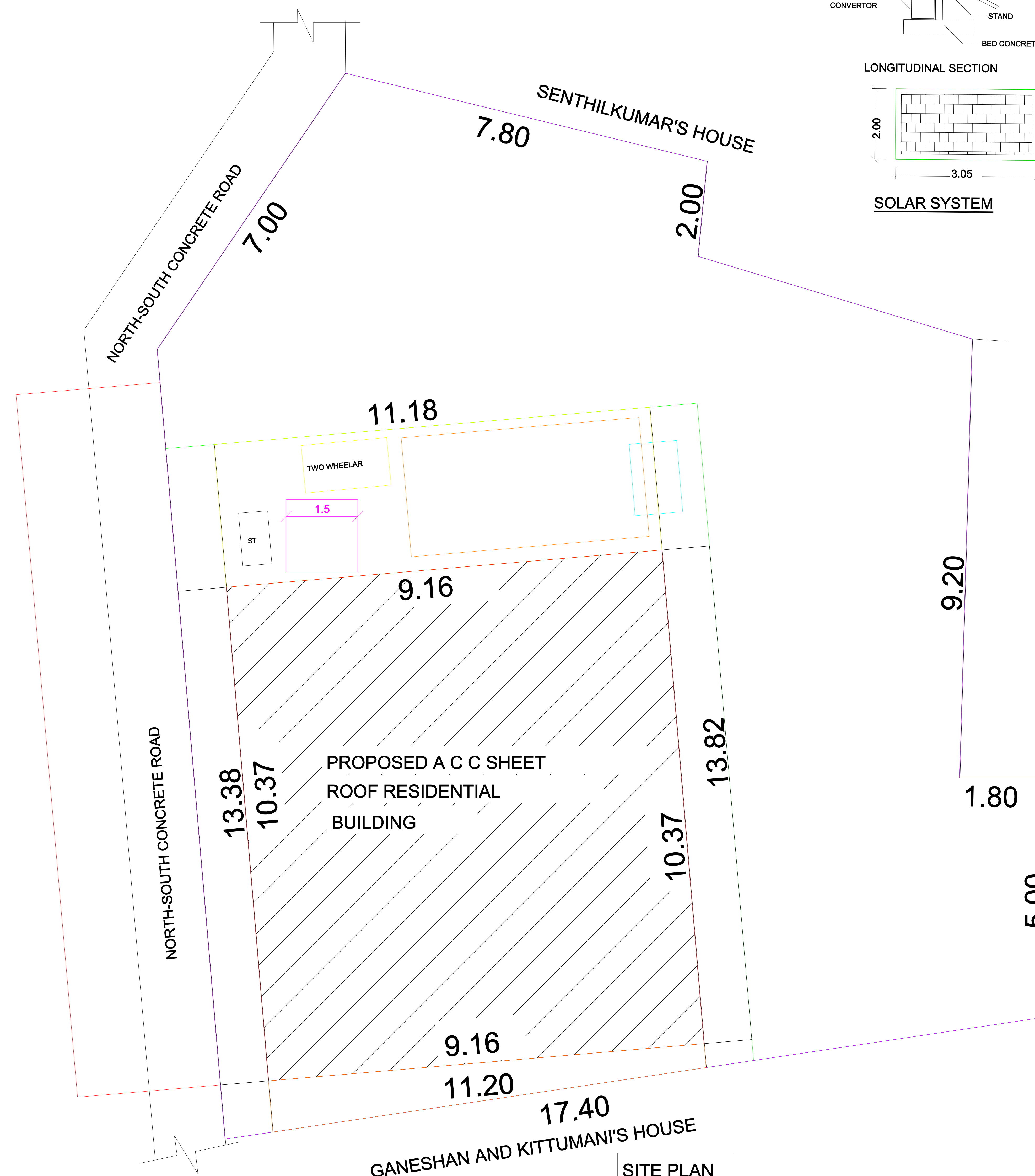
SITE PLAN
