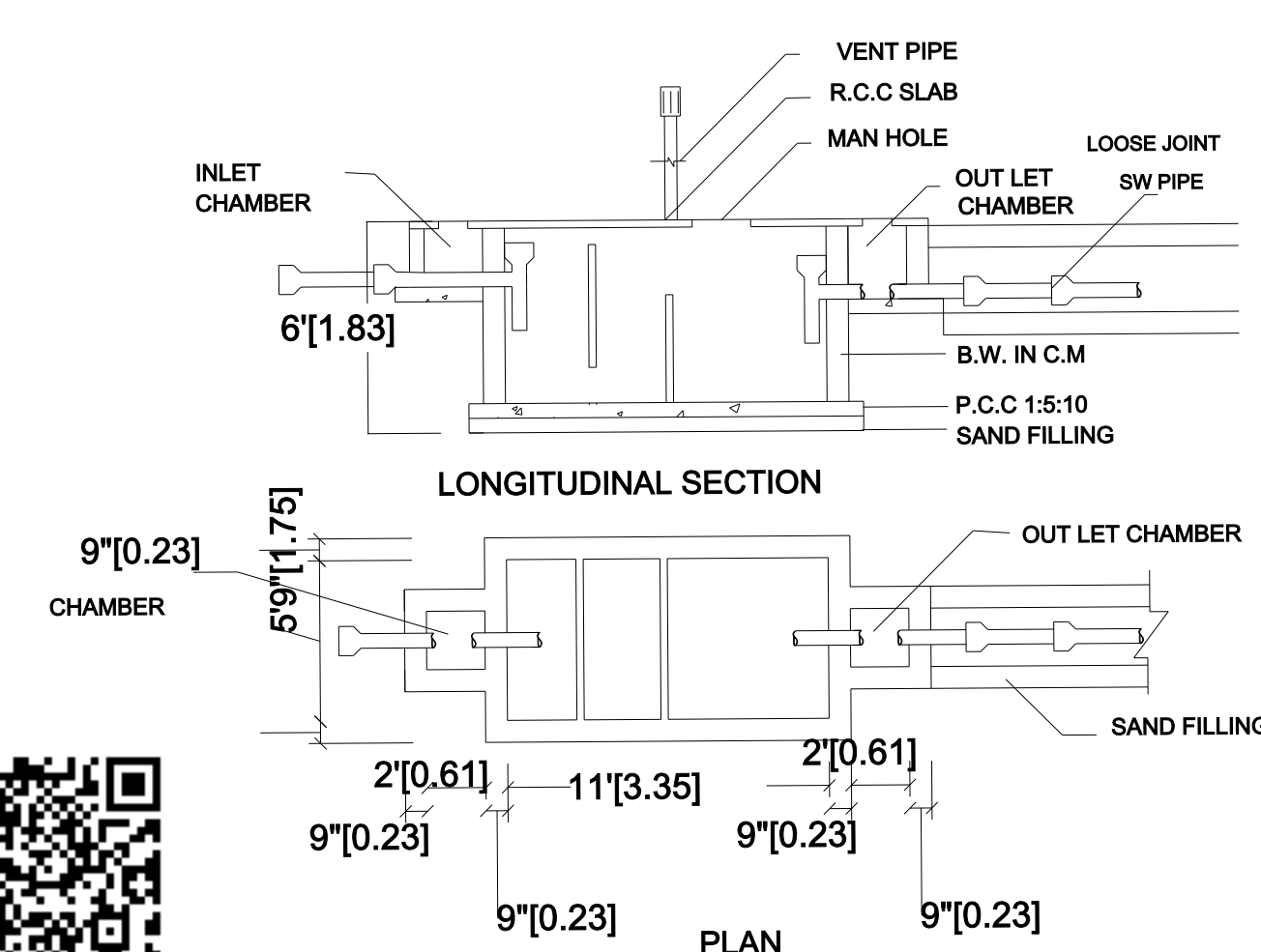
SEPTIC TANK:
