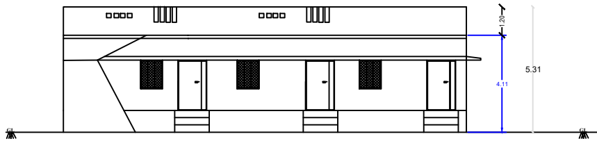
ELEVATION FACING EAST
