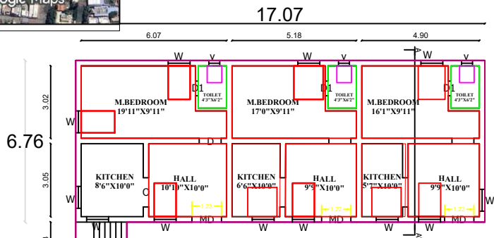
GROUND FLOOR PLAN FACING EAST
