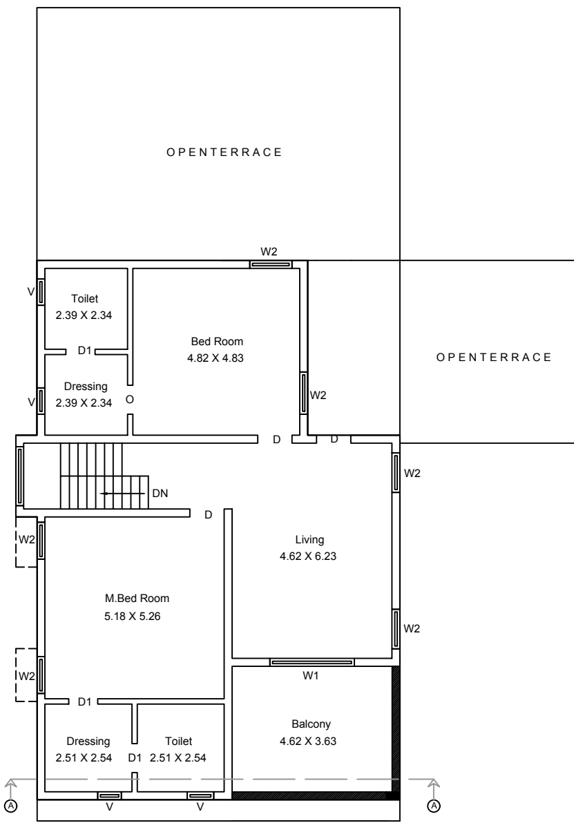
EXISTING FIRST & PROPOSED ADDITIONAL FIRST FLOOR PLAN
