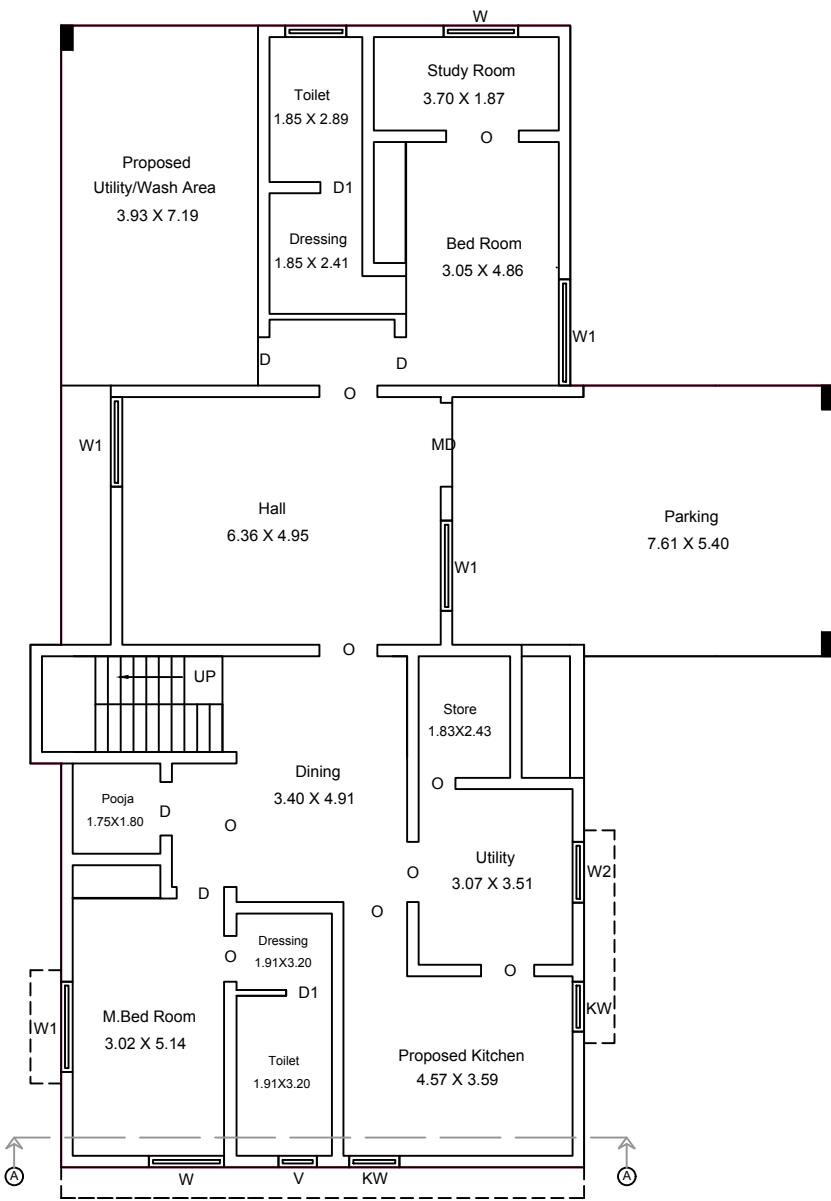
EXISTING GROUND & PROPOSED ADDITIONAL GROUND FLOOR PLAN
