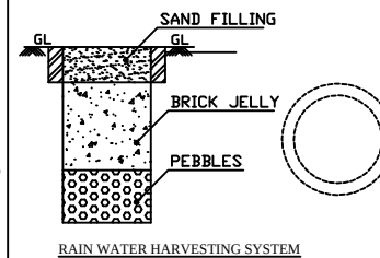
RAIN WATER HARVESTING SYSTEM
