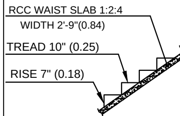
STAIRCASE DETAIL
