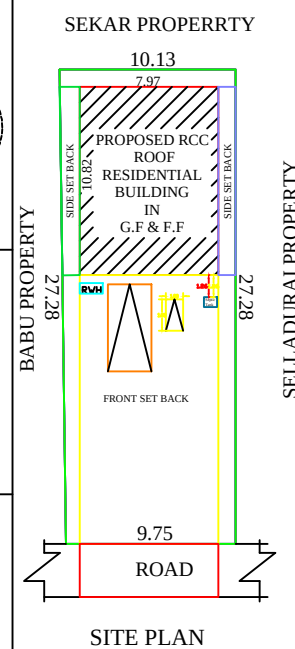
SITE PLAN
