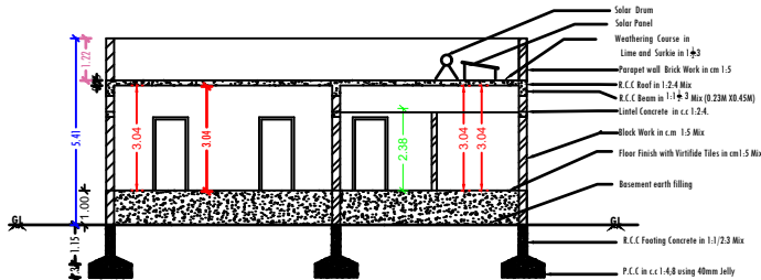
Section on "BC"
