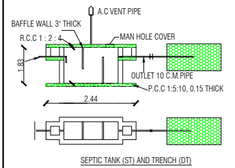
SEPTIC TANK (ST) AND TRENCH (DT)
