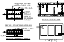
DETAILED DRAWING FOR SEPTIC TANK WITH DIFFERENTIAL TRENCH 225
