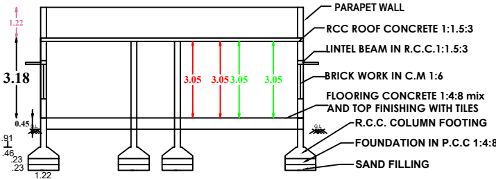
SECTION-AB
