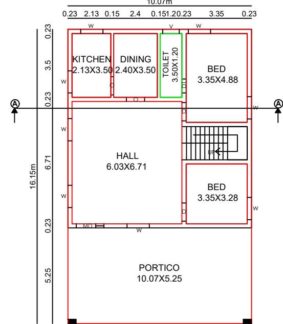
GROUND FLOOR PLAN (Facing on North)
