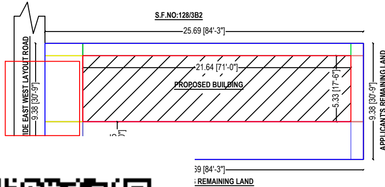
PROPOSED PLAN
