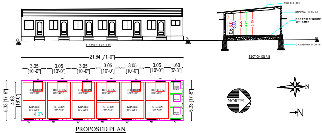
PROPOSED PLAN
