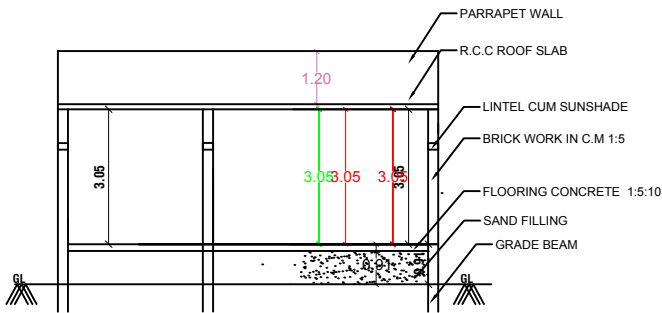
SECTION-AB
