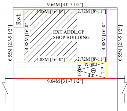
SITE PLAN (MEANT FOR CONSTRUCTION)
