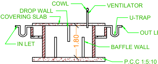
SEPTIC TANK DETAILS PLAN
