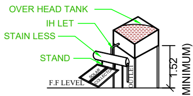
SOLAR WATER HEATING SYSTEM
