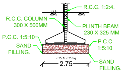
FOUNDATION DETAIL
