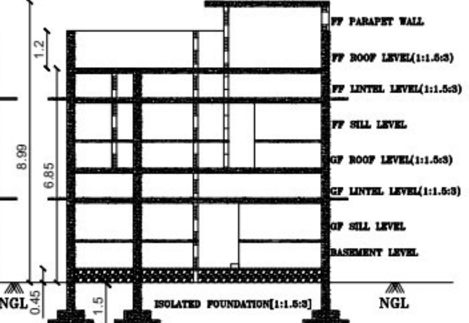
SECTIONAL VIEW ON A - A
