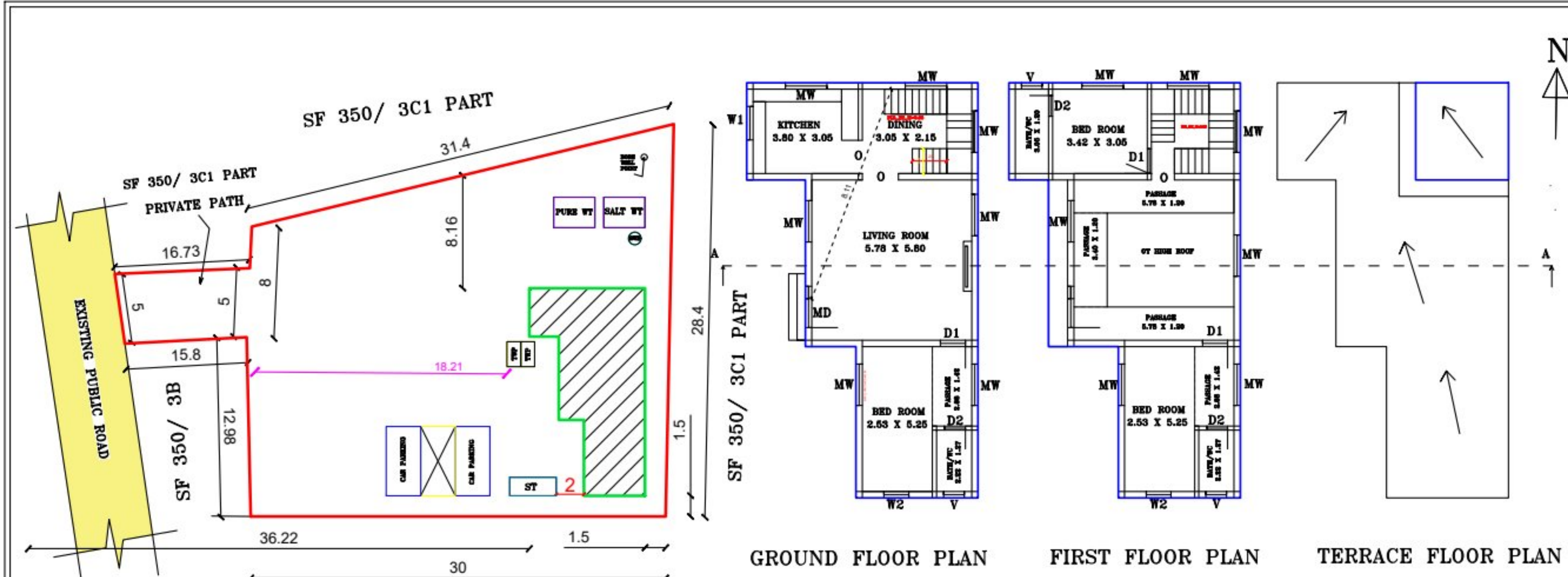
SF 350/ 3F,3C1 PART GROUND FLOOR BOUNDARY LINE DIAGRAM [ SCALE 1: 362 ]
