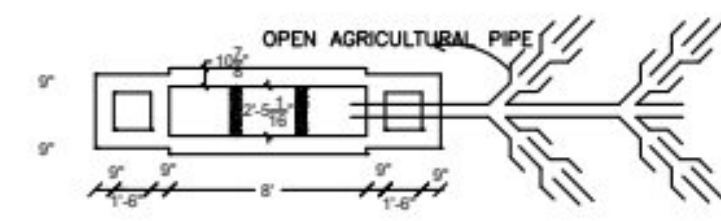
PLAN OF SEPTIC TANK DETAILS (SCALE : 0'1" = 6'0")
