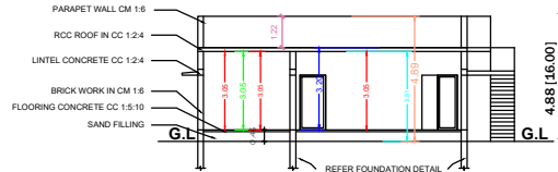
SECTIONAL VIEW -A-A'
