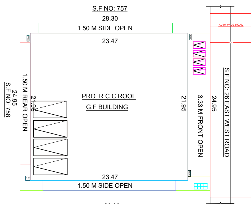
28.30 VASANTHAMANI'S PROPERTY SITE PLAN (SCALE 1:100)
