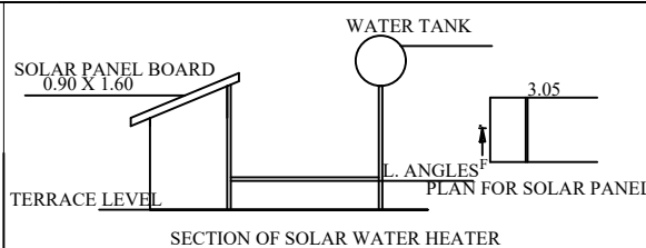
SECTION OF SOLAR WATER HEATER
