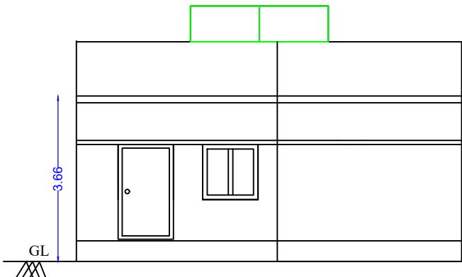
ELEVATION - NORTH
