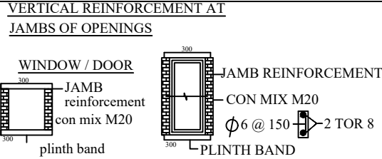
VERTICAL REINFORCEMENT AT JAMBS OF OPENINGS
