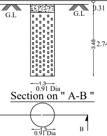
Detailed Plan of Rainwater Percolation and Collection Pit
