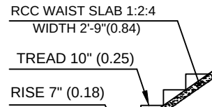
STAIRCASE DETAIL
