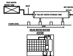
SOLAR HOT WATER SYSTEM DETAILS
