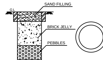
RAIN WATER HARVESTING SYSYTEM
