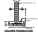
COLUMN FOUNDATION
