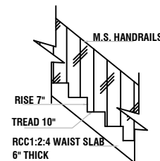
STAIRCASE DETAILS
