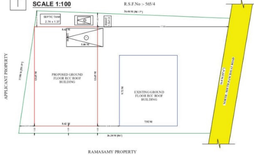
KEY PLAN
