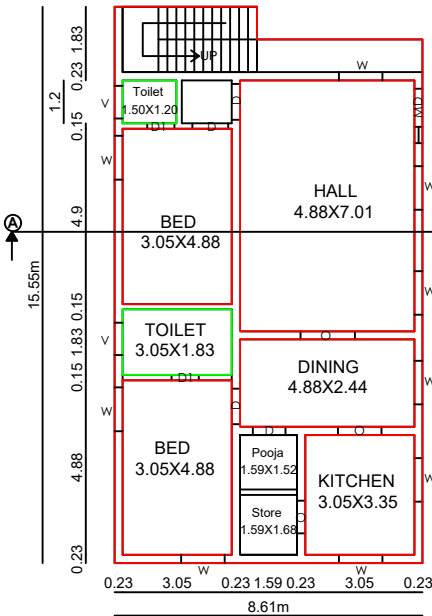
GROUND FLOOR PLAN (Facing on East)
