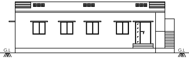
FRONT ELEVATION FACING ON EAST
