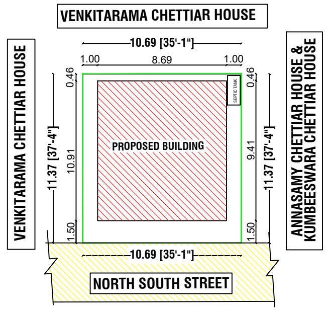
SITE PLAN
