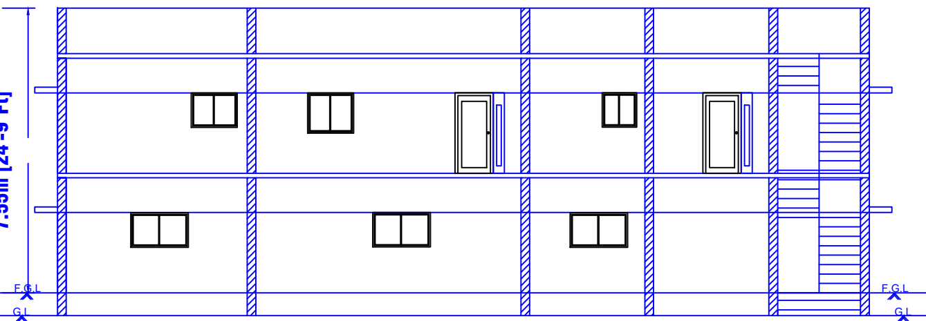
FRONT EAST FACING ELEVATION
