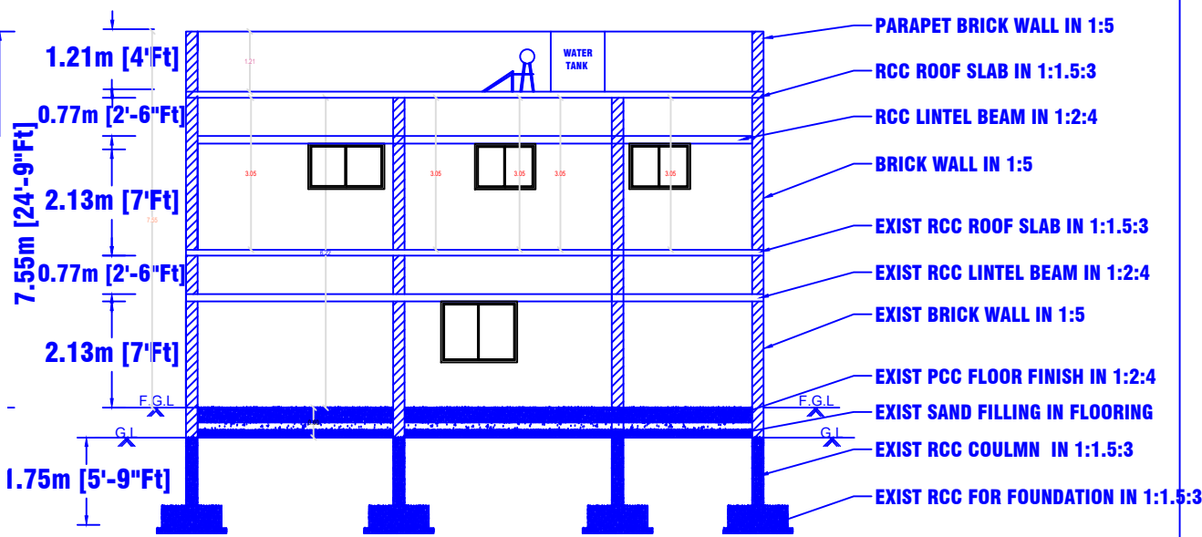
SECTION A - AA
