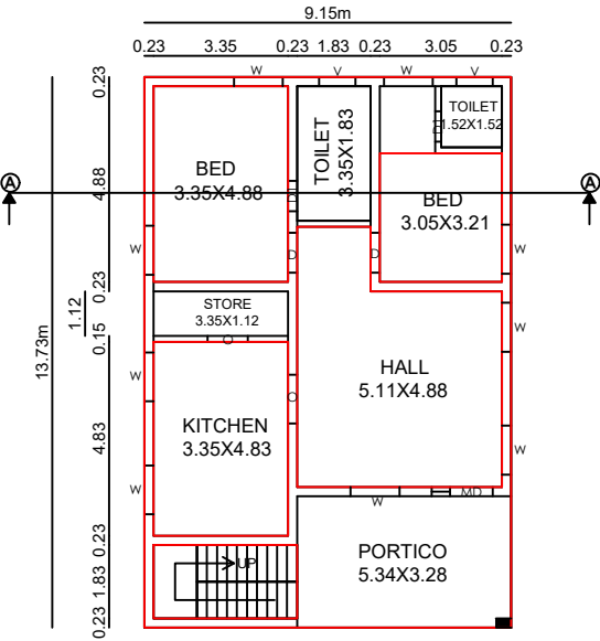
GROUND FLOOR PLAN (Facing on East)
