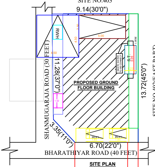
SITE PLAN
