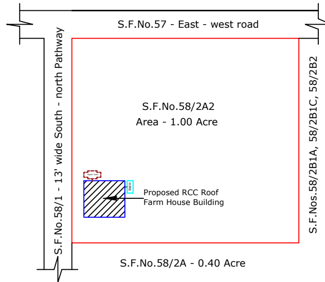
SITE PLAN
