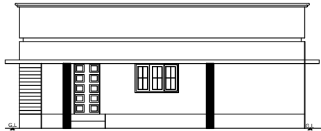
ELEVATION FACING NORTH
