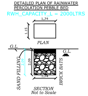
DETAILED PLAN OF RAINWATER PERCOLATION PEBBLE BED
