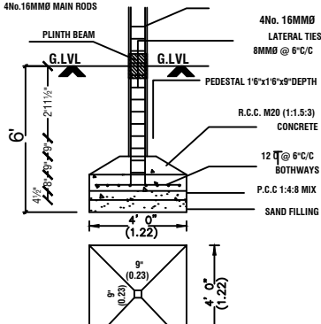
FOUNDATION DETAIL
