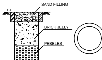
RAIN WATER HARVESTING SYSSTEM
