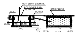
SECTION ON SEPTIC TANK & DISP-TRENCH
