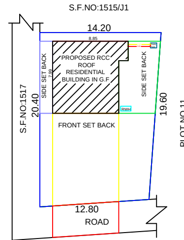
SITE PLAN
