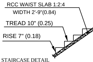
STAIRCASE DETAIL
