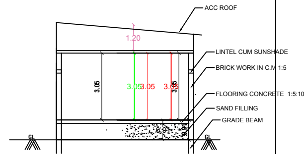
SECTION-AB
