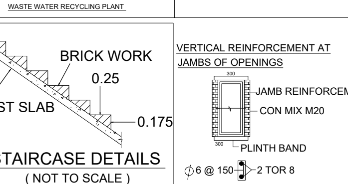
STAIRCASE DETAILS (NOT TO SCALE)
