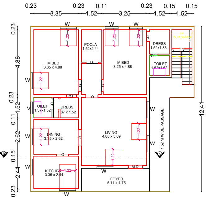
PRO.GROUND FLOOR (G.F) PLAN
