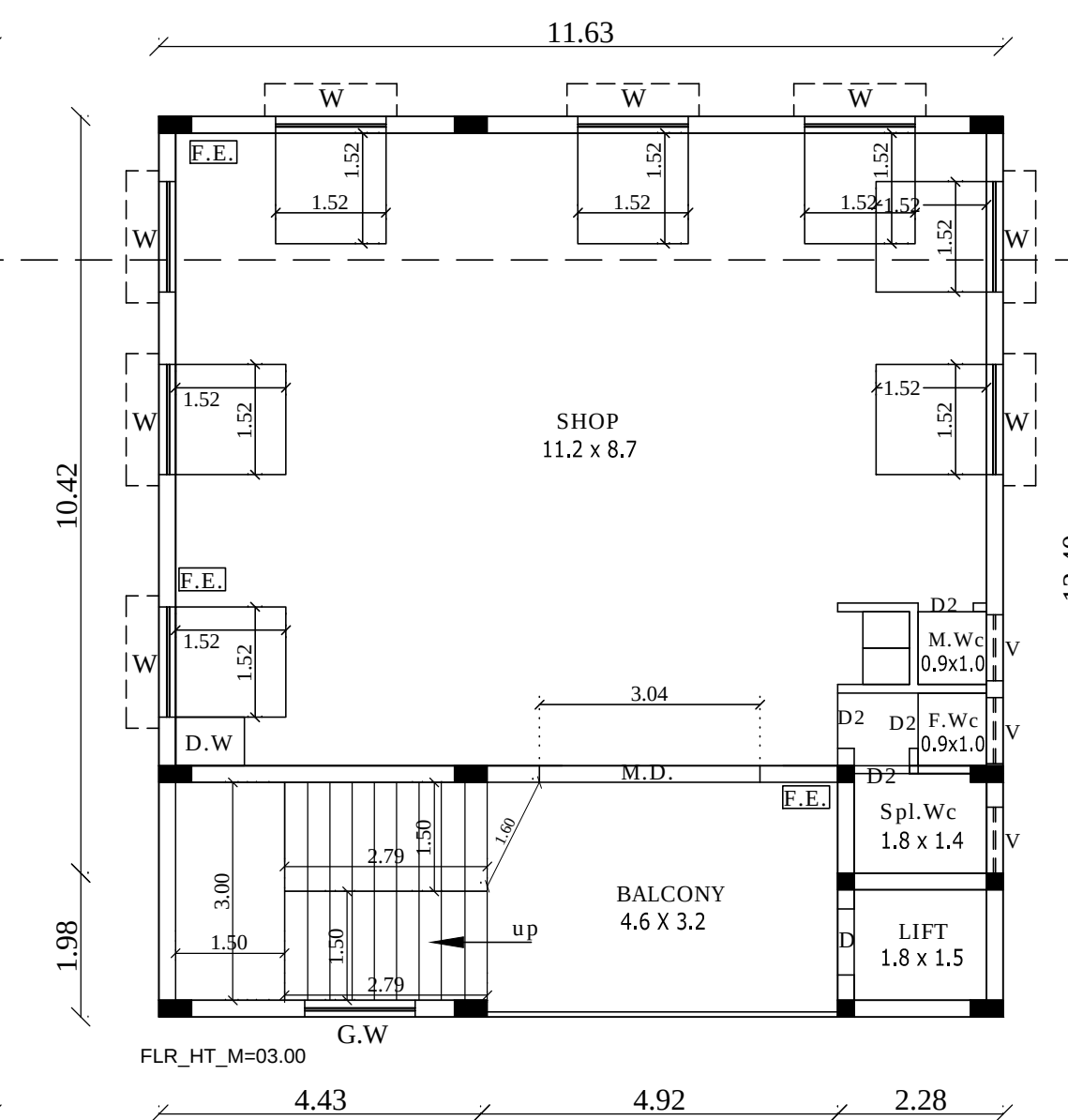
TYPICAL FIRST, SECOND &amp; THIRD FLOOR PLAN
