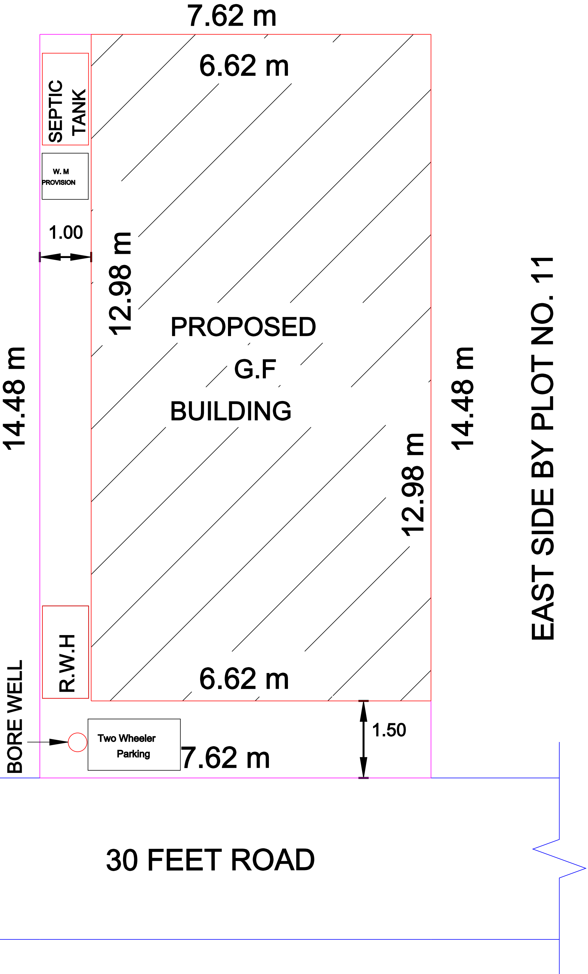
SITE PLAN
