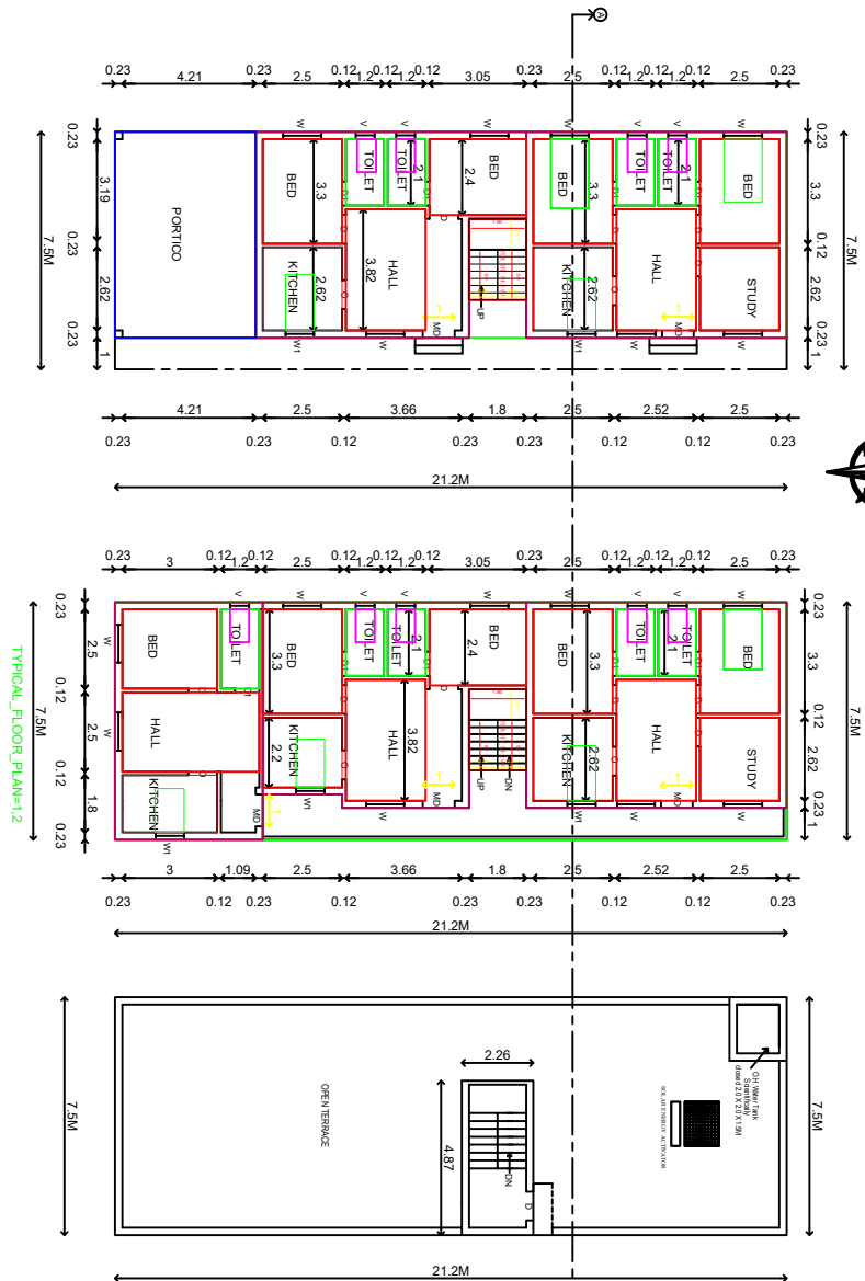
PRO.TERRACE FLOOR PLAN
