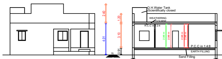
SIDE ELEVATION
