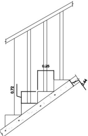
STAIRCASE DETAIL
