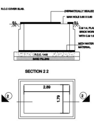
PLAN OF U.G SUMP (CAPACITY = 7800 lt)
