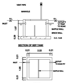
SEPTIC. TANK
