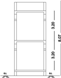
CROSS SECTION ON "AB"
