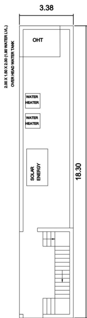
TERRACE FLOOR PLAN
