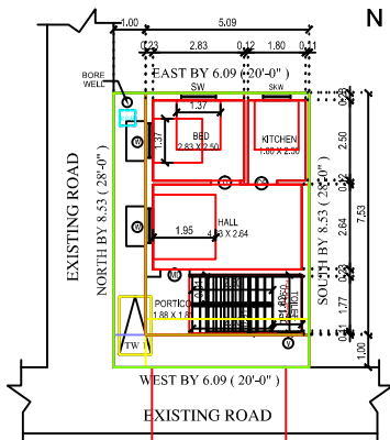
SITE CUM GROUND FLOOR PLAN
