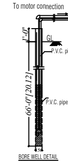
BORE WELL DETAIL
