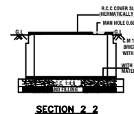
SECTION 2.2
