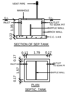
PLAN SEPTIC. TANK
