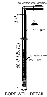
BORE WELL DETAIL
