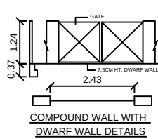
COMPOUND WALL WITH DWARF WALL DETAILS
