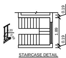
STAIRCASE DETAIL
