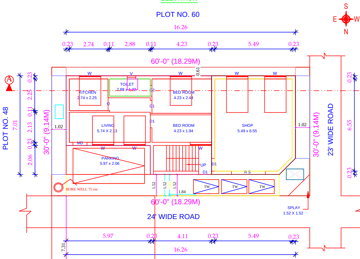
SITE CUM GROUND FLOOR PLAN
