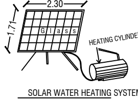
SOLAR WATER HEATING SYSTEM SCALE:1:30
