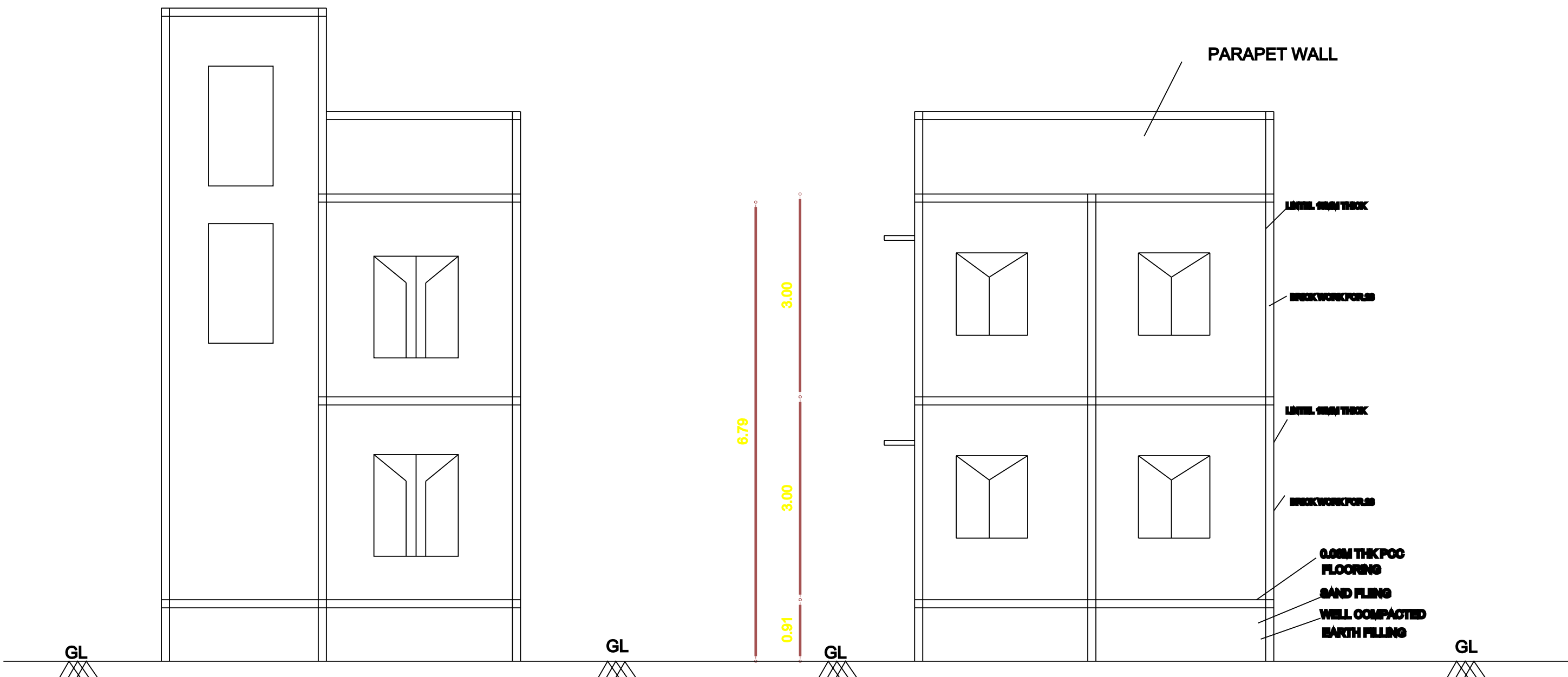
SECTION-AA
