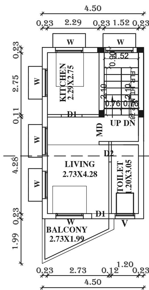
FIRST FLOOR PLAN ( PROPOSED )
