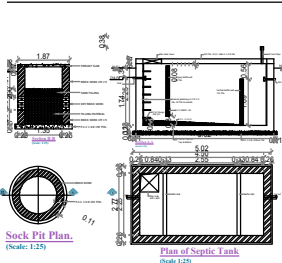
SEPTIC TANK
