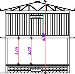
SECTION ON A-A
