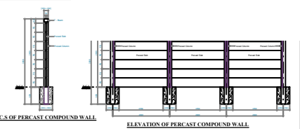
ELEVATION OF COMPOUND WALL
