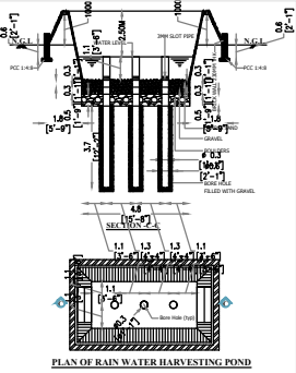
PLAN OF RAIN WATER HARVESTING POND
