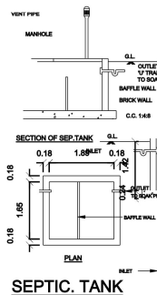
SEPTIC TANK
